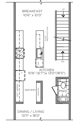
PART. SECOND FLOOR OPT. KITCHEN LAYOUT
