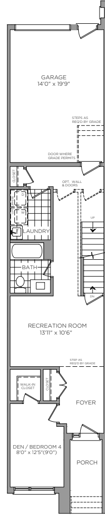
FIRST FLOOR ELEVATION A/B
