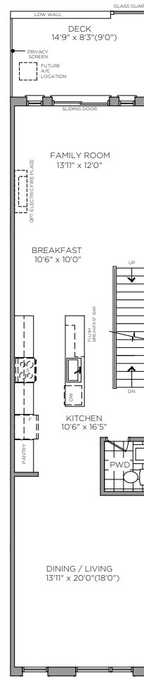
SECOND FLOOR ELEVATION A/B
